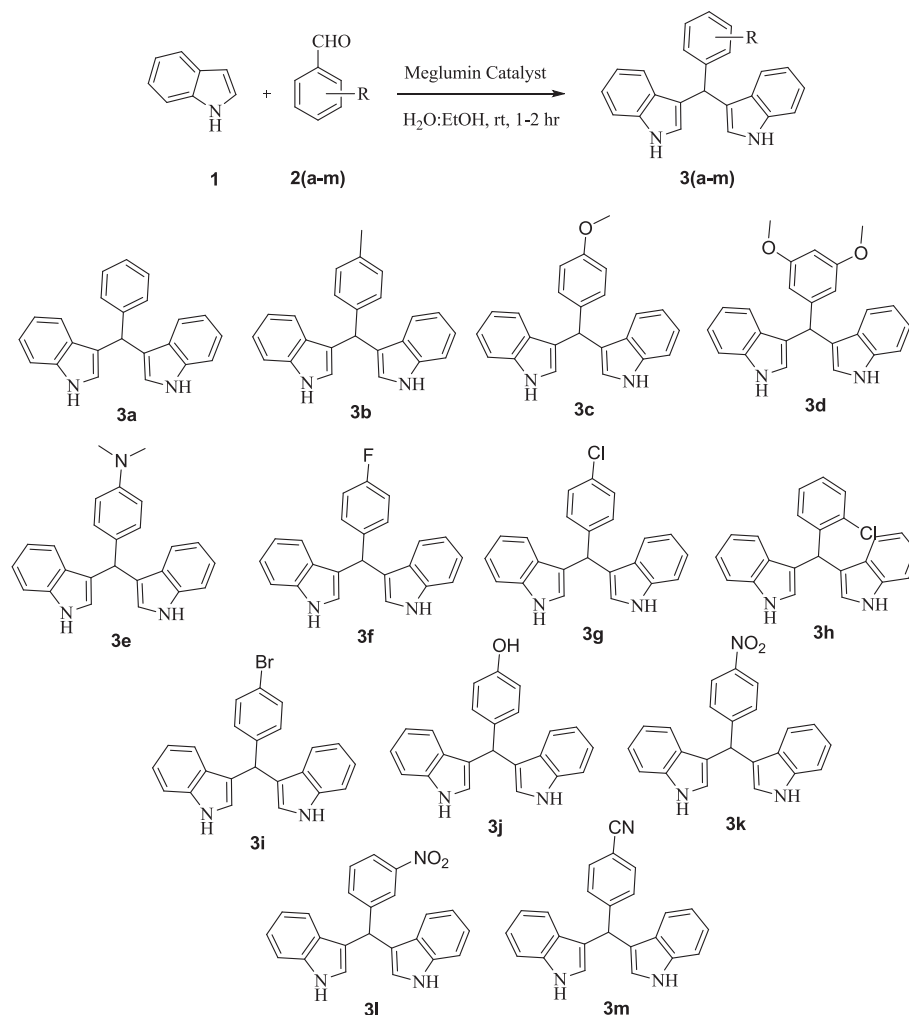
SCHEME 1 Synthesis of bis(indolyl)methane derivatives ( 3a-m )
