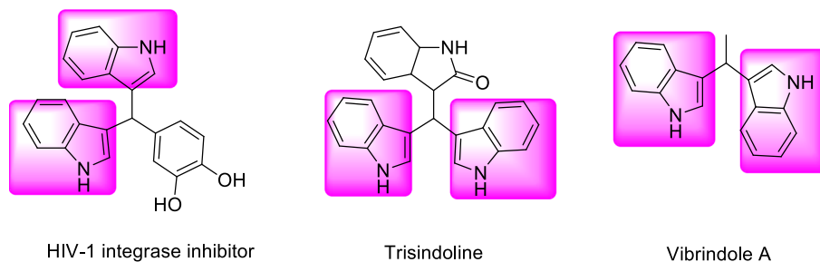
FIGURE 1 Bio-active BIMs derivatives [Color figure can be viewed at wileyonlinelibrary.com ]
